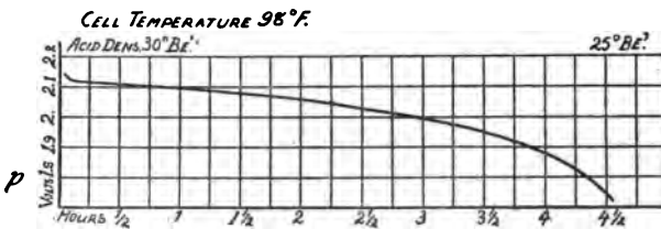
FIG. 31 a .—Discharge Curve of First Discharge in 4½ hours at 20 amperes of a 5 plate, 9-inch cell used for ignition, showing very gradual fall in voltage through ⅔ of the period.
